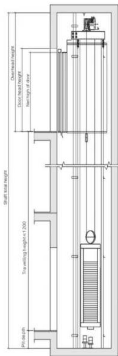
Models B750 and B1000 hoistway and machine room elevation
