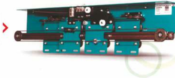
4-Panel Centre Opening Landing Door Mechanism
