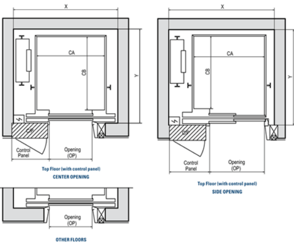
HOISTWAY PLAN
